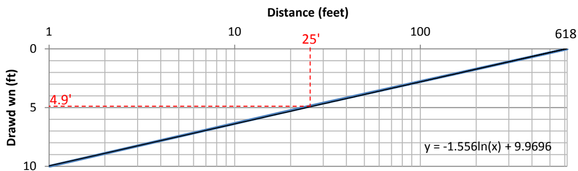
Figure 4: Semi-log Plot of Drawdown vs. Distance
