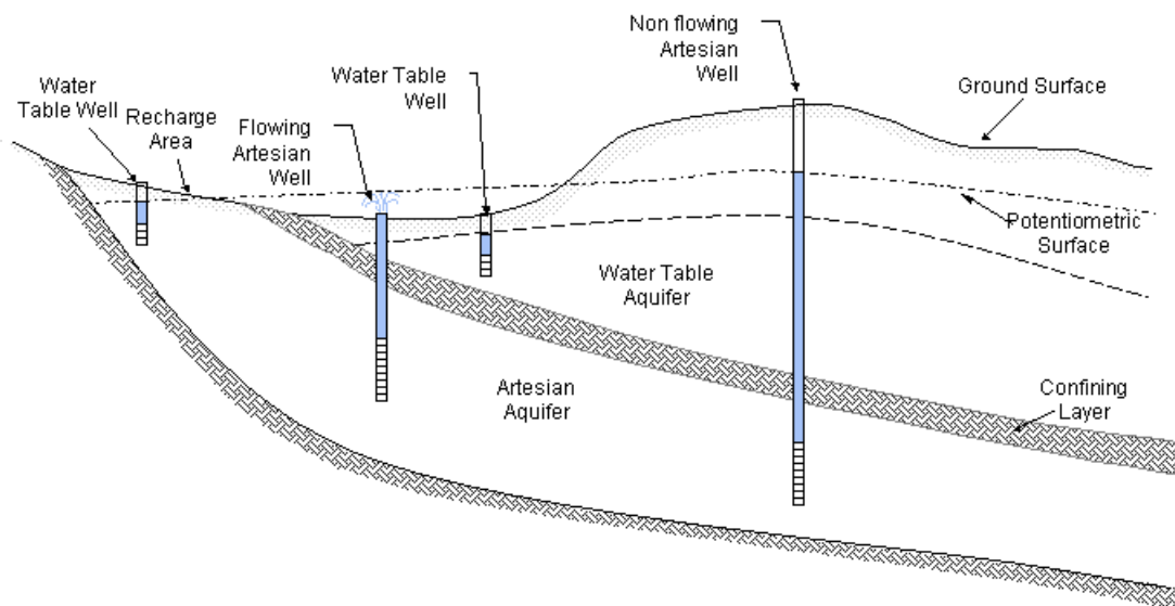
Figure 3: Confined Aquifer (artesian flow conditions) Adapted from FHWA, "Highway Subdrainage Design"
