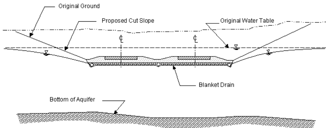
Figure 6: Drainage Blanket System Adapted from FHWA, "Highway Subdrainage Design"
